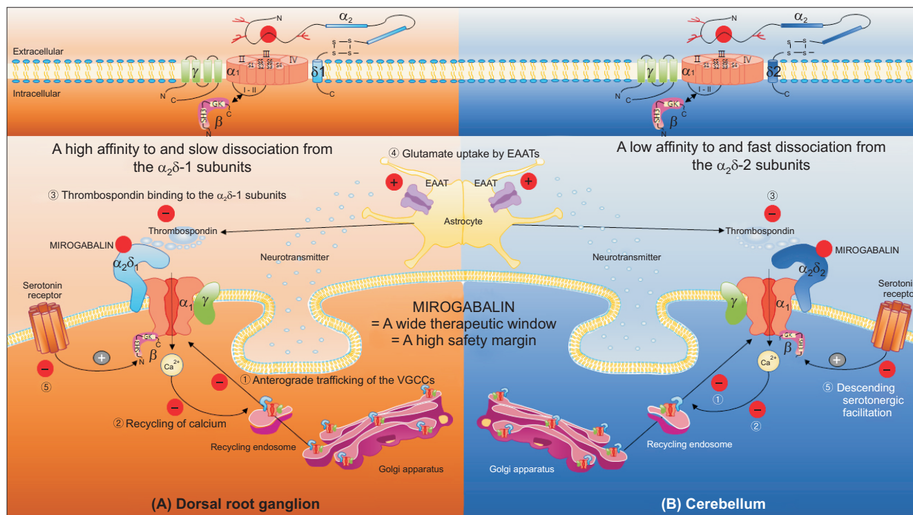
Fig. 1. A schematic illustration of the mechanisms of action for mirogabalin. Mirogabalin has a high affinity to and slow dissociation from the \alpha_2\delta -1 subunits in the dorsal root ganglia (DRGs), producing greater therapeutic effects; it also has a low affinity to and fast dissociation from the \alpha_2\delta -2 subunits in the cerebellum, producing lesser adverse drug reactions. In general, various mechanisms of action for gabapentinoids are suggested from inside the cell, membrane, and synapse. (1) Gabapentinoids inhibit forward (anterograde) trafficking of voltage-gated calcium channels (VGCCs) (from the endoplasmic reticulum through the Golgi complex to the cell membrane) intracellularly. Inhibition of anterograde trafficking reduces VGCCs, calcium entry, and excitatory amino acids (glutamates). (2) They inhibit the Rab-11-dependent final recycling of endosomal VGCCs intracellularly, resulting in reduced excitatory neurotransmitter release in the synapse. The small guanosine triphosphatases (GTPases, Rab) are the main regulators of intracellular membrane trafficking, from formation of transport vesicles to their fusion into the membranes. Reduced recycling of endosomal VGCCs results in reduced transmembrane VGCCs, calcium entry into the cell, and glutamate in the synapse. (3) They inhibit astrocyte-derived thrombospondin (TSP, extracellular matrix protein)-mediated excitatory synapse formation extracellularly (reduction of excitatory synaptogenesis). (4) They stimulate glutamate uptake by excitatory amino acid transporters (EAATs) extracellularly. (5) Gabapentinoids may show inhibition of descending serotonergic facilitation, stimulation of descending inhibition, anti-inflammatory effect, and influence on the affective component of pain. A magnified illustration for the transmembrane VGCC is shown in the upper left (in the DRGs) and right (in the cerebellum) quadrants. Adapted from Chincholkar M. Analgesic mechanisms of gabapentinoids and effects in experimental pain models: a narrative review. Br J Anaesth 2018; 120: 1315-34 [14].
