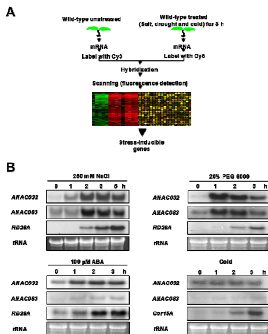
Fig. 1. Microarray preparation and Northern blot analysis. (A) A schematic performing of microarray analysis for multi abiotic stress inducible genes. (B) Confirmation of isolated ANAC genes under abiotic stresses by Northern blot analysis. Seven-day-old Arabidopsis wild-type seedlings were exposed to NaCl (250 mM), PEG (20%), ABA (100 \mu M), or cold (4 ^{\circ} C) for indicated time period.
