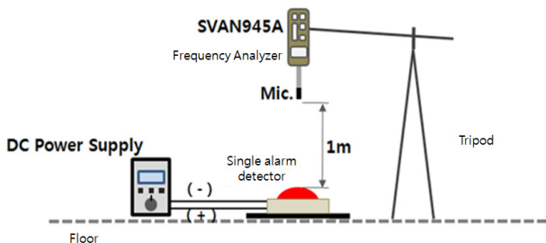
Figure 1. Schematic diagram of sound pressure level measurement according to voltage change.
