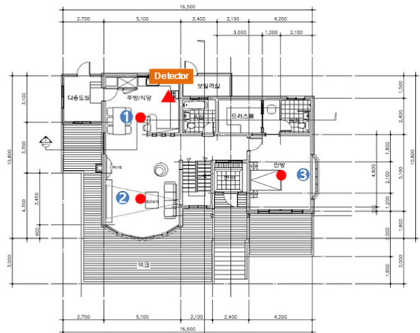
a) Floor plan of 1 st floor
