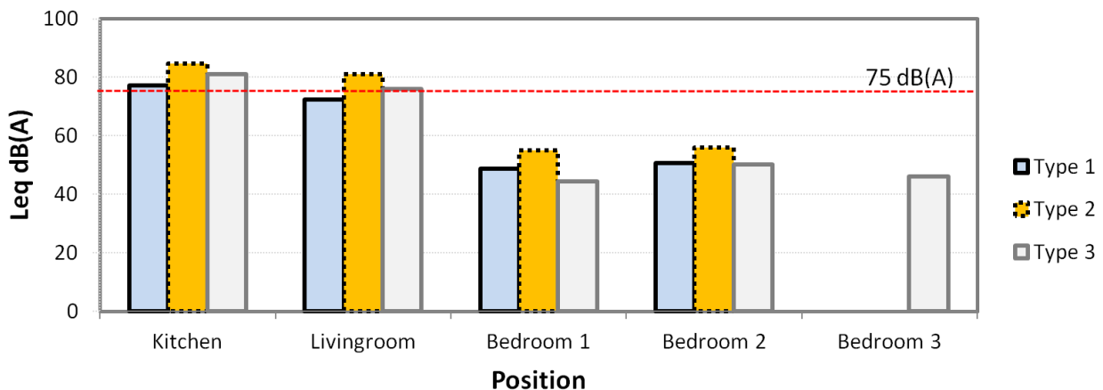
Figure 6. Predicted Sound Pressure Level (dBA) in Each Indoor Space by House Type.
