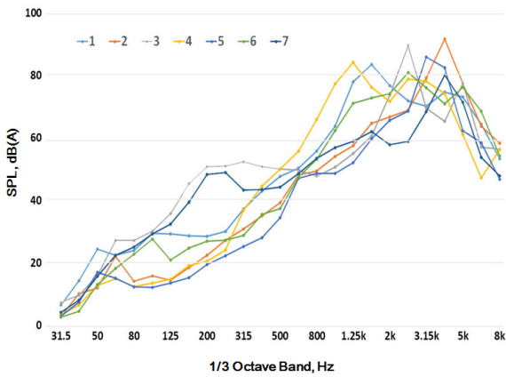
Figure 2. Spectral characteristics of sound pressure level measured at 1m when the alarm sound of the detector occurs.
