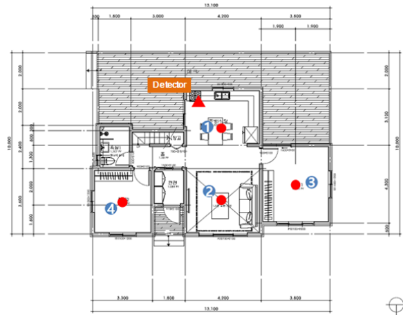
Figure 4. Detector location (▲) and masturbation point location (●) for Type 2 house.
