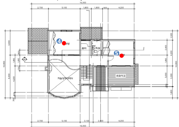
b) Floor plan of 2 nd floor
