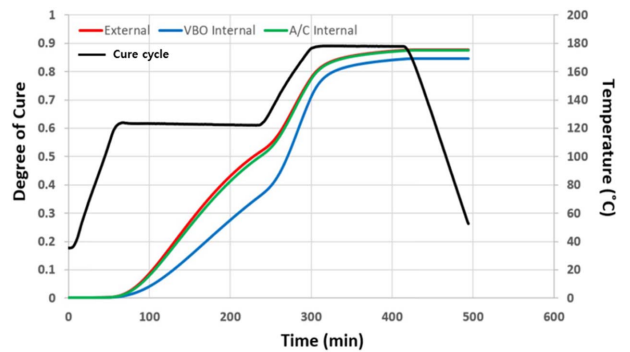
Fig. 8. Cure kinetics simulation at Option #1
