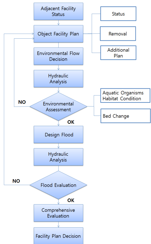
Fig. 8. Result of Hydraulic Analysis by Design Flood Discharge
