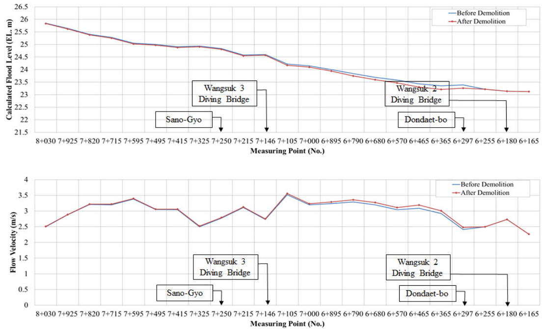
Fig. 5. Result of Hydraulic Analysis before and after Dondaet-bo Demolition by Design Flood Discharge
