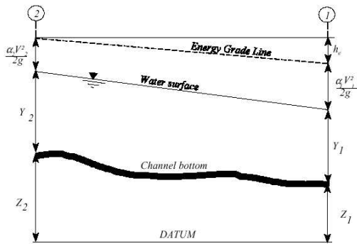
Fig. 2. Diagram of Energy Equation
