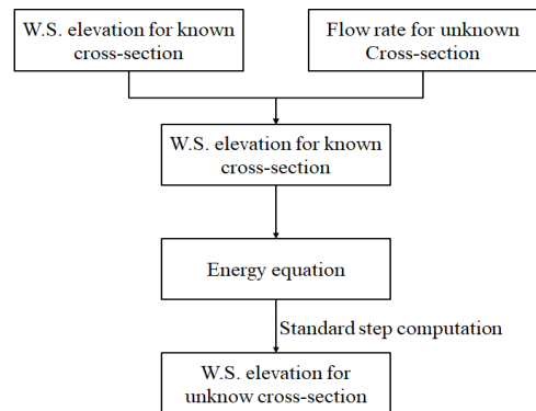
Fig. 1. Computational Process of HEC-RAS
