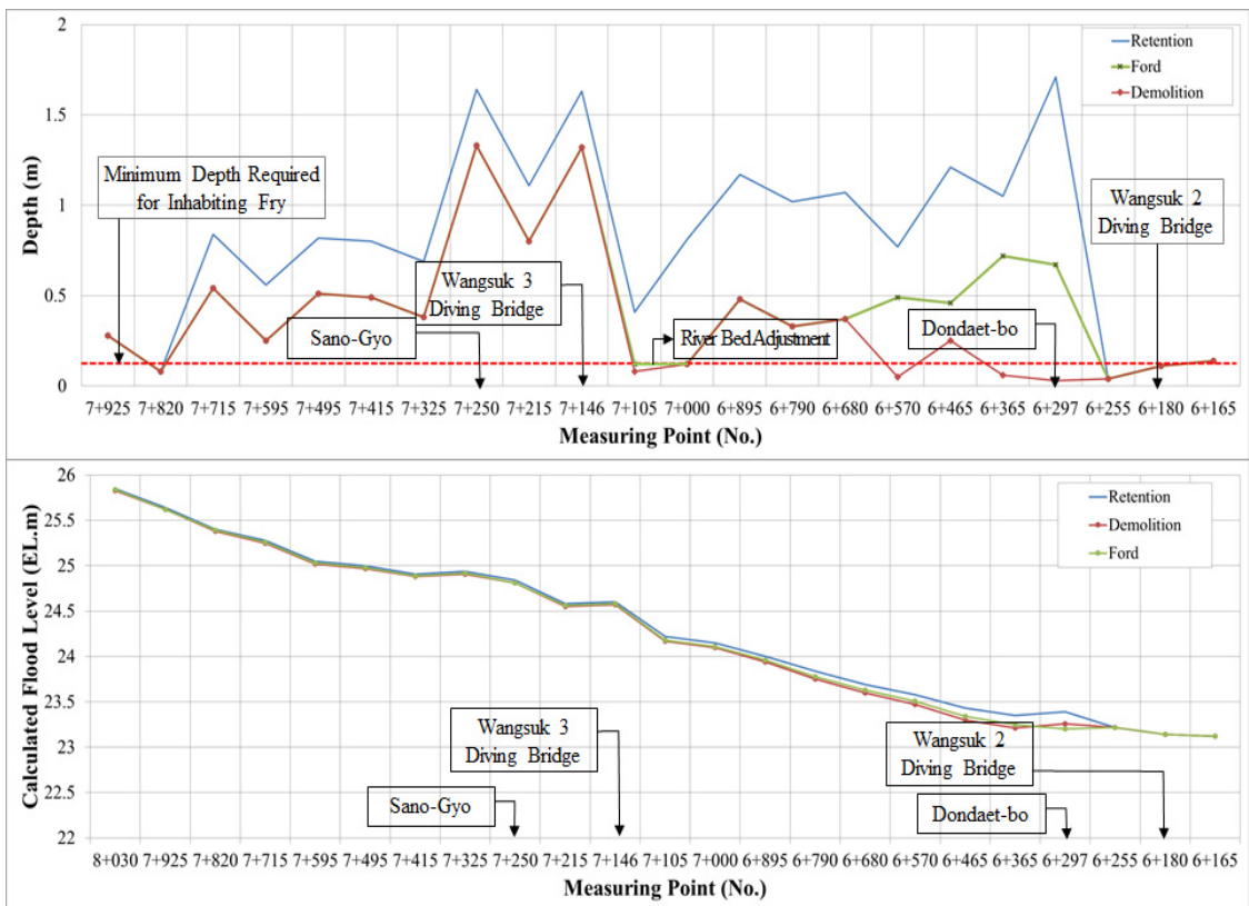
Fig. 7. Result of Hydraulic Analysis Using Environmental Flow after Installing Natural Riffle
