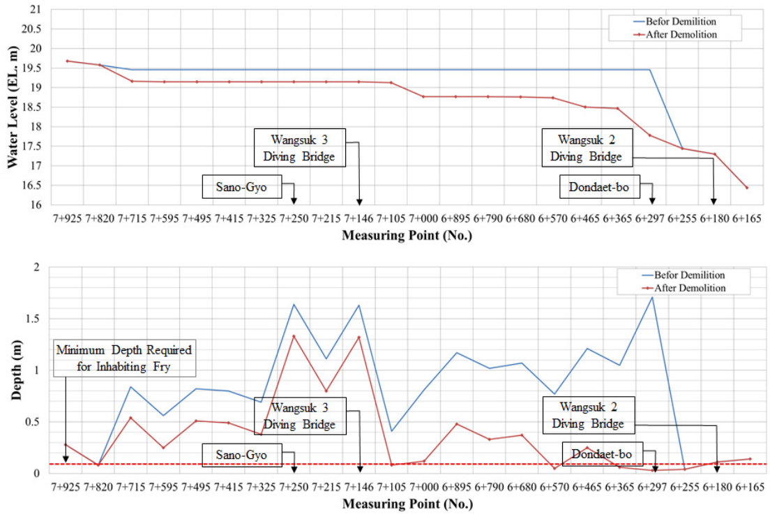
Fig. 4. Result of Hydraulic Analysis before and after Dondaet-bo by Environmental Flow
