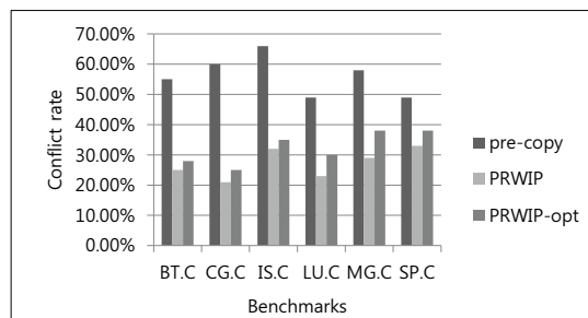
Fig. 10. Conflict rate (checkpoints interval is 5 seconds).
