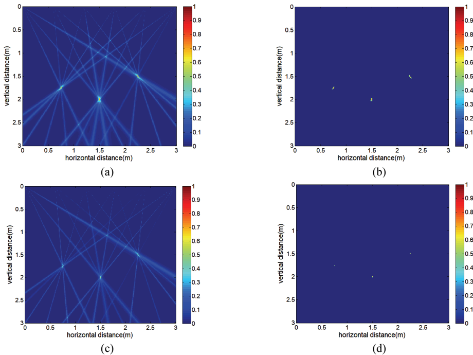
Fig. 4. Localization of multi-targets with SNR=0 dB, (a) original image of reverse projection of Capon algorithm, (b) image of adding threshold of Capon algorithm, (c) original image of reverse projection of MUSIC algorithm, (d) image of adding threshold of MUSIC algorithm.
