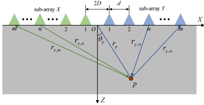
Fig. 1. Model of GPR based on two symmetric sub-arrays.
