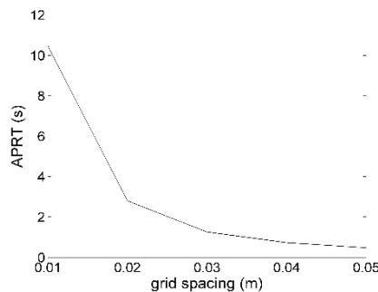
Fig. 5. Relationship between APRT and grid spacing (under the Inter i7-6700 processor using MATLAB R2013a).
