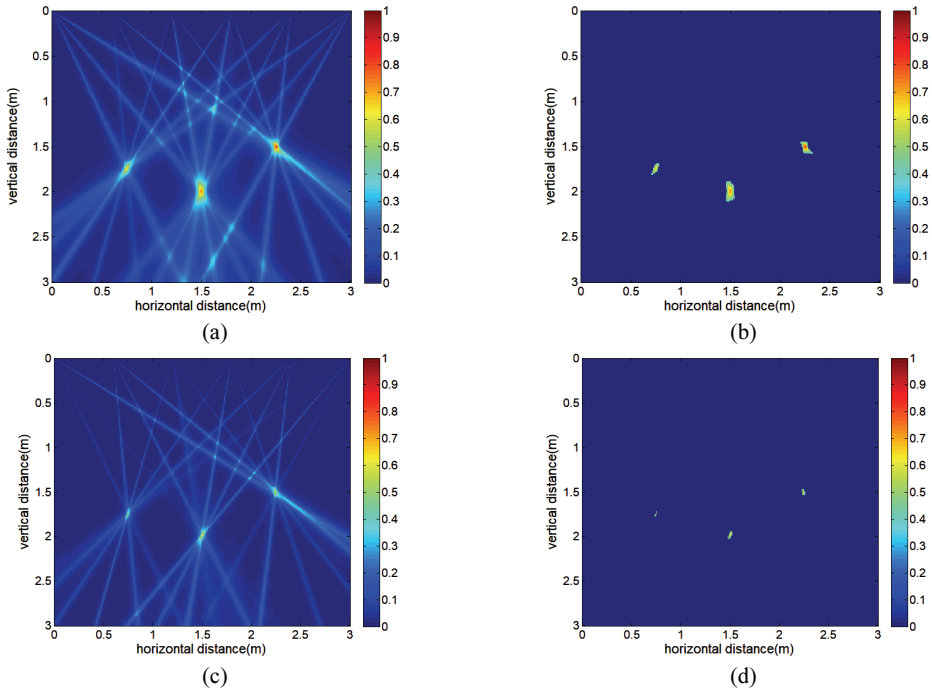
Fig. 3. Localization of multi-targets with SNR=-10 dB: (a) original image of reverse projection of Capon algorithm, (b) image of adding threshold of Capon algorithm, (c) original image of reverse projection of MUSIC algorithm, and (d) image of adding threshold of MUSIC algorithm.
