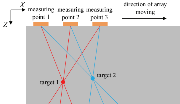
Fig. 2. Principle diagram of target localization by reverse projection.
