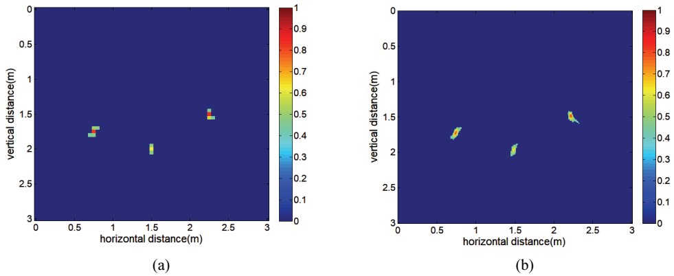
Fig. 6. Localization of multi-targets of Capon algorithm with SNR = -10 dB: (a) low-resolution imaging the entire area of \Delta d = 0.05 m and (b) high-resolution of the target area of \Delta d = 0.01 m.
