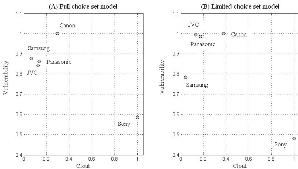
<Figure 5> Clout and vulnerability charts implied by the full consideration set (panel A) and consideration set (panel B) models. Note that all the values are normalized for comparison purposes within charts (A) and (B)
