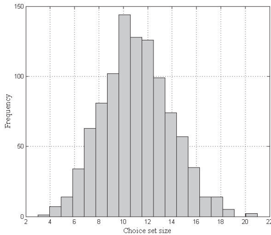
⟨Figure 3⟩ Histogram of the consideration set sizes from simulations at t=1 with l=1,000 consumers
