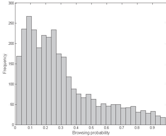
〈Figure 2〉 Histogram of browsing probabilities approximated from the view-list data across products and time
