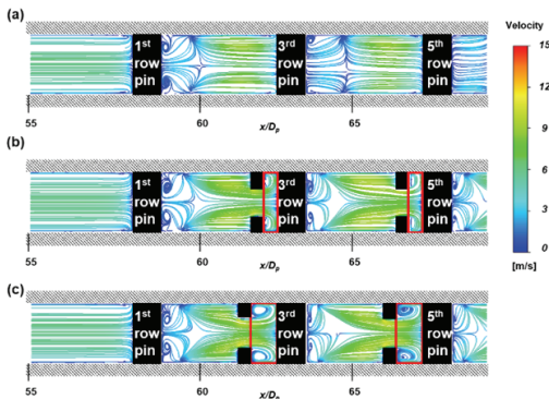
Fig. 5 Flow distributions at y/D_p=0 plane; (a) base case (b) cut pin case 1 and (c) cut pin case 2.
