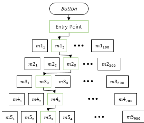
Fig. 4. Possible dummy flow from dummy entry point to real entry point
