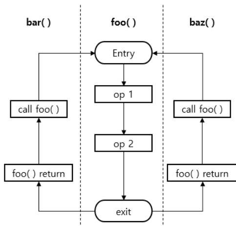
Fig. 1. Example of inter-procedural control flow graph. This graph is consists of 1 main procedure and 2 extra procedures.
