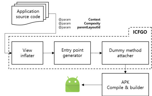
Fig. 2. Overall architecture and obfuscation pipeline of ICFGO
