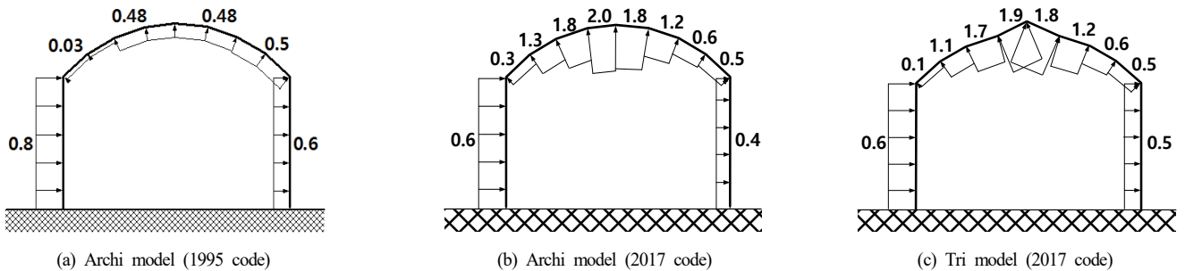
Fig. 5. External pressure coefficient of plastic greenhouse
