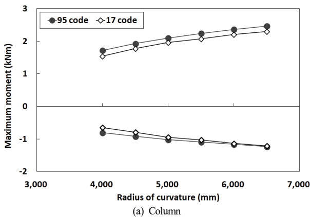
Fig. 3. Maximum moment of elements for wind load
