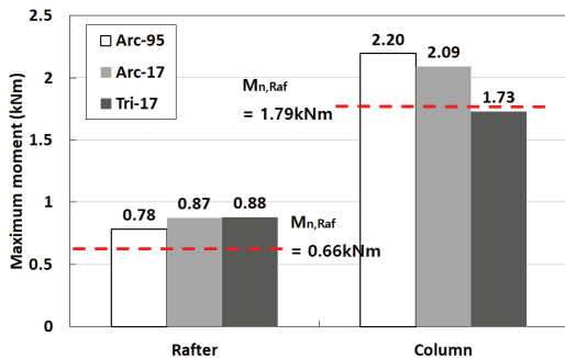
Fig. 6. Analysis results for original model
