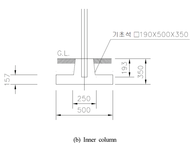
Fig. 10. Details of footing of type-1 house
