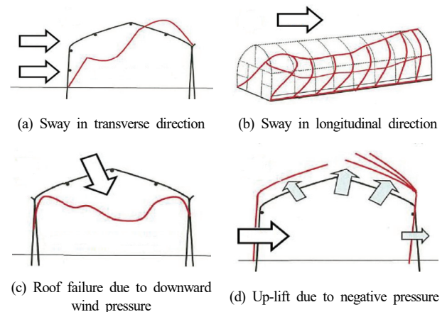
Fig. 1. Failure mode of plastic greenhouse
