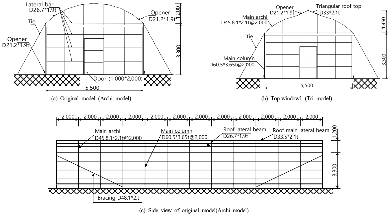
Fig. 4. Drawings of plastic greenhouses
