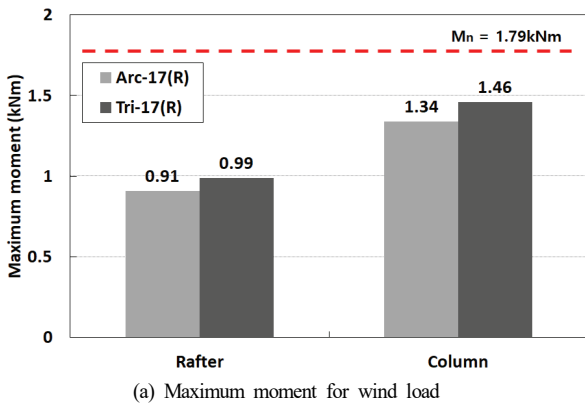
Fig. 9. Analysis results for original model
