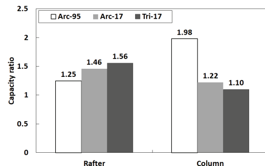
Fig. 6. Analysis results for original model
