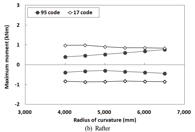
Fig. 3. Maximum moment of elements for wind load
