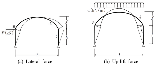
Fig. 7. Bending moment diagram for arch frame
