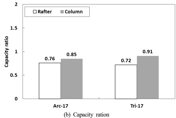
Fig. 9. Analysis results for original model
