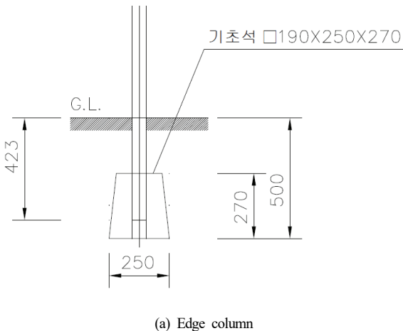
Fig. 10. Details of footing of type-1 house
