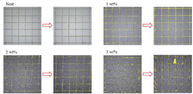
Fig. 7. Photographs of CNT/PU topcoat after cross hatched cut test
