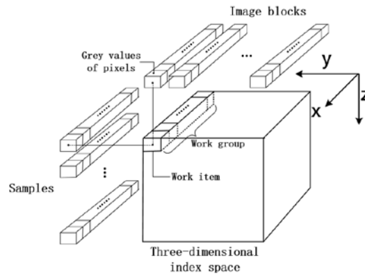
Fig. 9. OpenCL index space for NCC Calculation.
