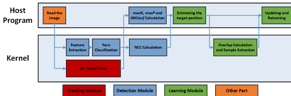
Fig. 3. The framework of our parallel TLD based on OpenCL. Most compute-intensive modules are implemented and optimized in kernel functions. Others are still processed in host program.
