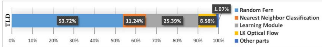
Fig. 2. Execution time distribution for all modules in TLD. The compute-intensive modules in TLD include random fern, learning module, nearest neighbor classification.
