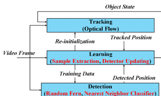
Fig. 1. TLD is composed of three parts, tracking, detection and learning. Tracking module is implemented by optical flow. Learning module includes sample extraction and detector updating. Detection module is composed of random fern and nearest neighbor classifier. Most recent LT trackers [17-19] are inspired by or derived from the structure of TLD.
