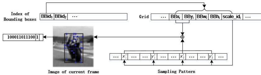
Fig. 5. Fern Feature Extraction.
