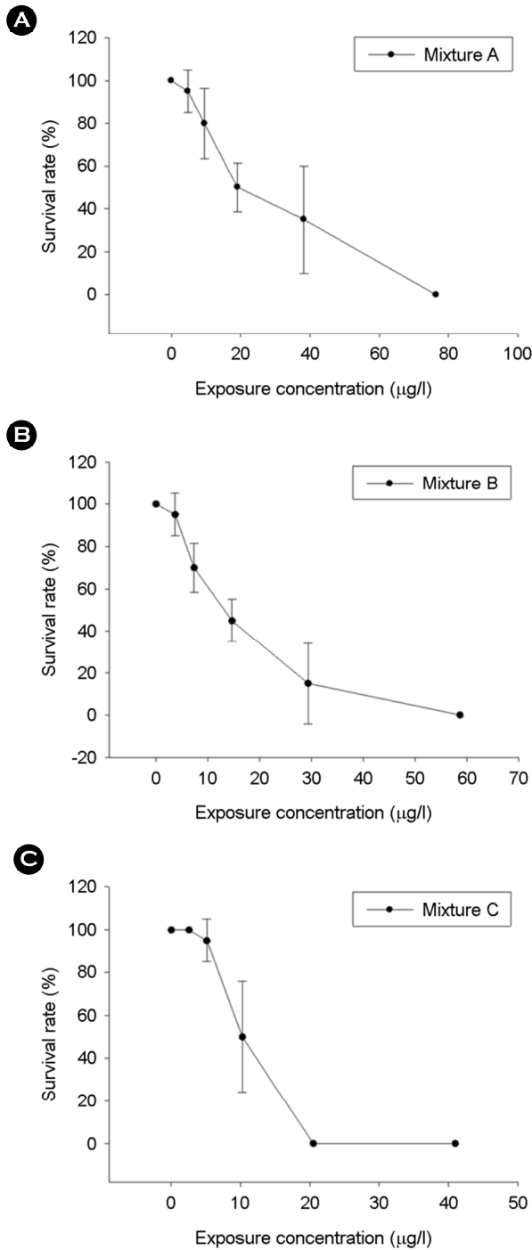
Fig. 2. Survival rate of Diaphanosoma celebensis exposed to (A) mixture A (3:7), (B) mixture B (5:5), (C) mixture C (7:3) of Benzo[a]pyrene and HgCl 2 for 48 h. Data are mean ± standard deviation (S. D.).
