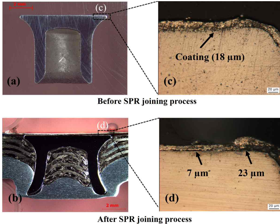
Fig. 4 Cross-sections of rivet (a) as received condition, and (b) after joining process of CFRP to Al joint, (c) and (d) magnified view of rivet head coating as received condition and after joining process, respectively.
