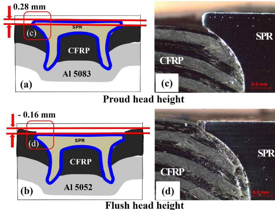
Fig. 6 Cross-sections schematic of CFRP to Al alloy SPR joints with (a) proud head, and (b) flush head, (c) and (d) magnified view of proud head and flush head joints, respectively.
