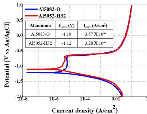
Fig. 13 Potentiodynamic polarization curve of Al5083-O and Al5052-H32 aluminum alloys.
