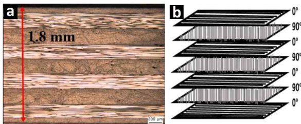
Fig. 2 CFRP laminate (a) cross-section, and (b) schematic of uni-directional prepreg orientation.
