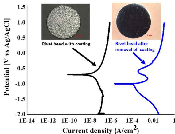
Fig. 16 Potentiodynamic polarization curve of rivet head (with Almac ® coating and after removal of coating).
