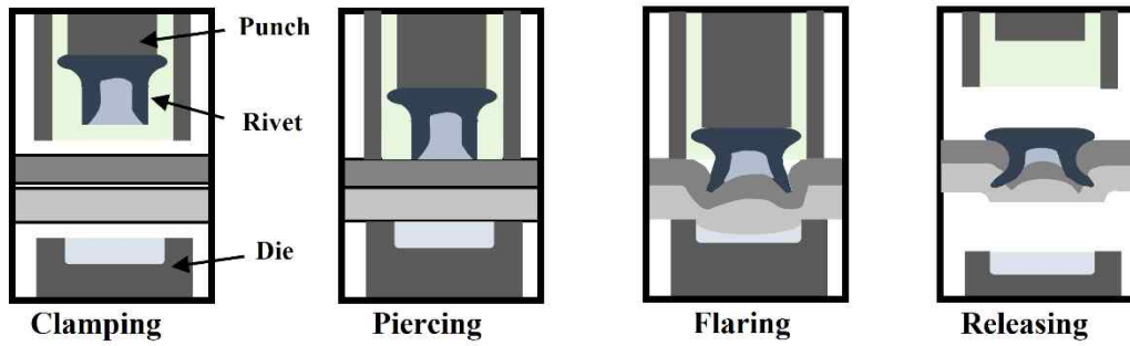
Fig. 1 Schematic diagram of four stages of SPR process.
