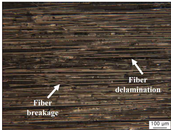
Fig. 14 Fiber breakage and delamination by removal of CFRP top ply.
