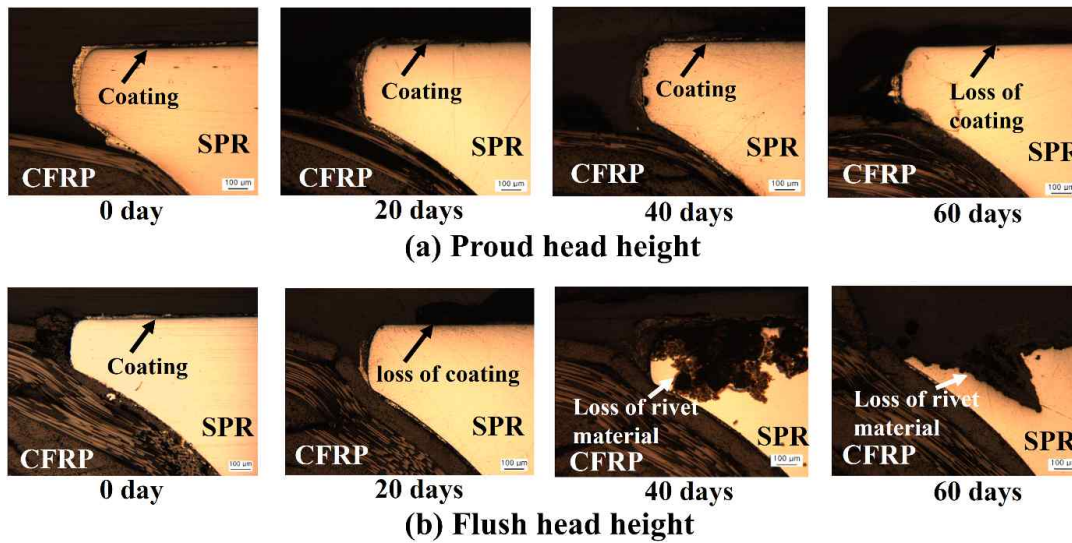
Fig. 11 Cross-section of rivet head at initial condition, and corrosion in 20, 40 and 60 days of salt spray test of (a) proud head height, and (b) flush head height.
