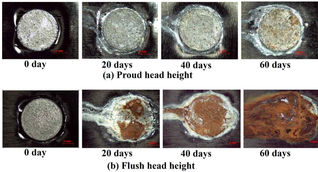
Fig. 7 Corrosion morphologies of rivet head for different salt spray test time of (a) proud head height, and (b) flush head height.
