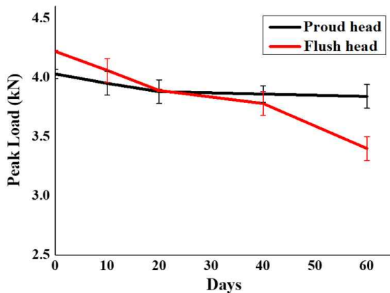
Fig. 9 Shear load for proud head and flush head SPR joints in different aged salt spray test time.
