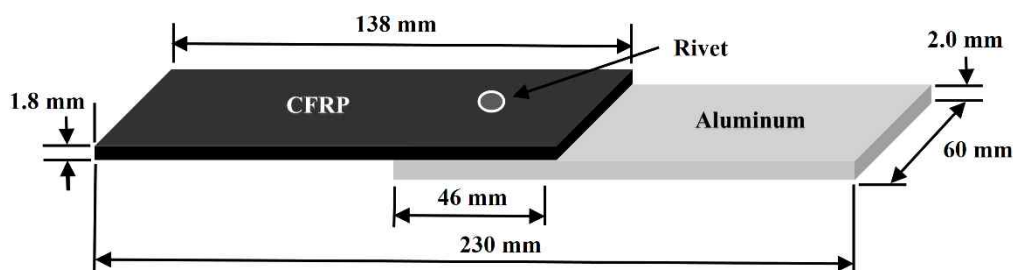
Fig. 3 Schematic of lap shear SPR joint geometry.
