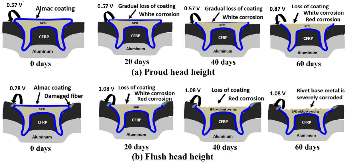
Fig. 17 Schematic diagram of corrosion mechanism of rivet head at different aging time for (a) proud head height, and (b) flush head height.
