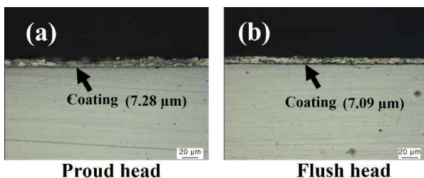
Fig. 5 Coating thickness on rivet head after SPR joining process of (a) proud head height (b) flush head height.
