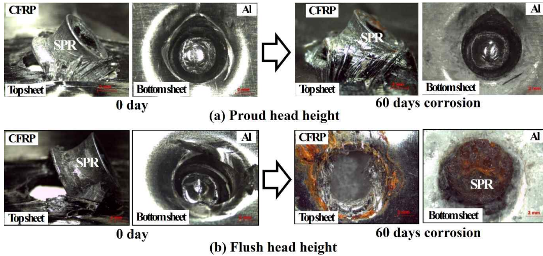
Fig. 10 Failure mode at initial condition and 60 days aged corrosion of (a) proud head height, and (b) flush head height.
