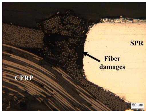
Fig. 12 CFRP breakage and delamination around the rivet head by flush head SPR joint.
