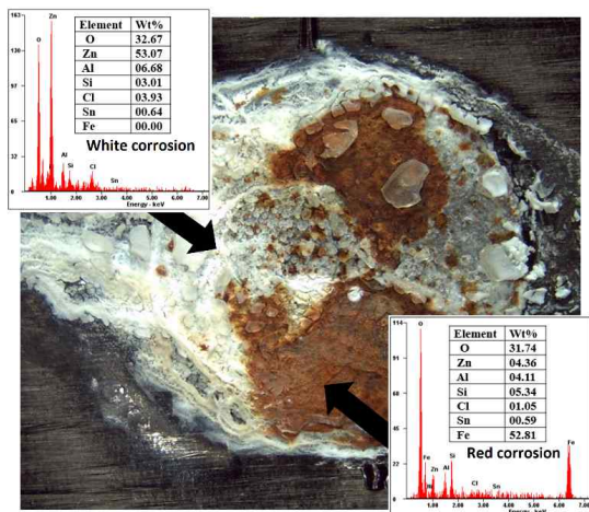
Fig. 8 Energy-dispersive X-ray analysis (EDXA) analysis for white and red corrosion product characterization on rivet head.
