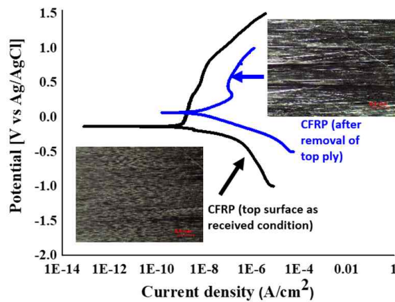
Fig. 15 Potentiodynamic polarization curve of CFRP (top surface of received condition and after removal of top ply).
