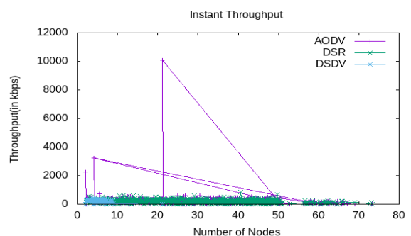
Fig. 3. Instant Throughput v/s Number of nodes.
