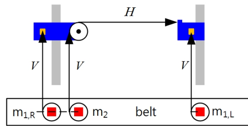
[Fig. 12] Modeling of the cart position, cable length and the distance between carts
