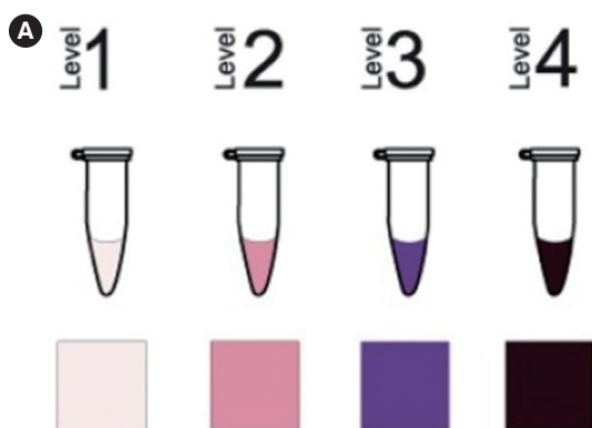
Figure 1. (A) Reactive oxygen species (ROS) intensity color scheme for semen samples using the Oxisperm kit assay. The figure was supplied by halotech (Madrid, Spain). (B) ROS intensity plot for the infertile and fertile samples using the Oxisperm kit assay. L (level) 1, low; L2, low-medium; L3, medium; L4, high.
