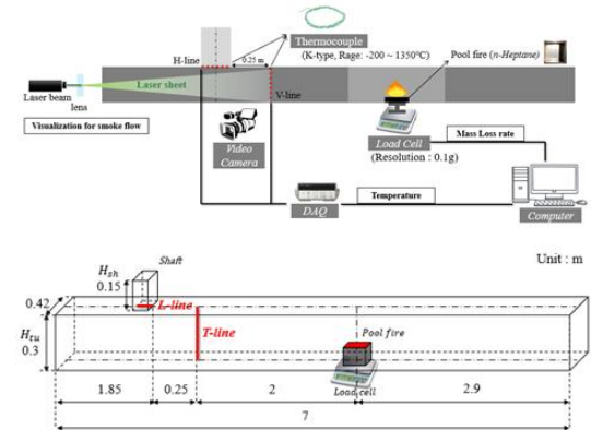
Fig. 1. The schematic of the reduced tunnel.
