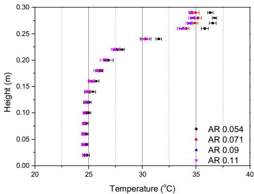
Fig. 3. Transverse temperature distribution in tunnel. (Pool area 20.25 cm 2 )
