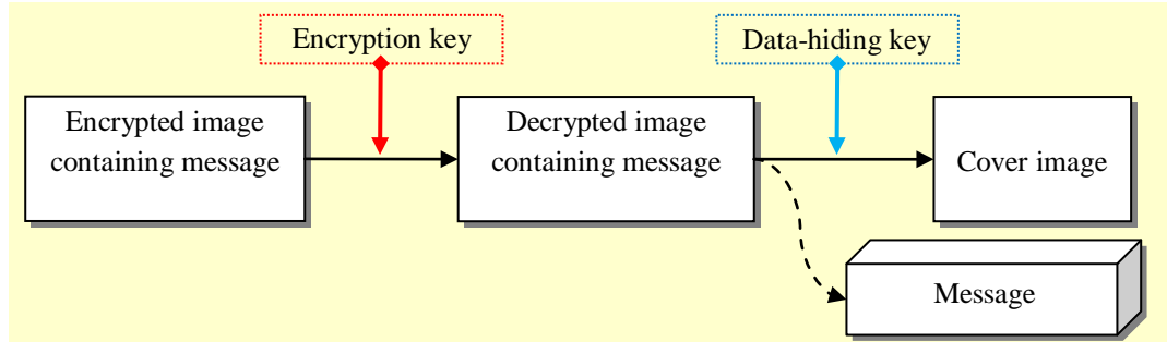
Fig. 2. Receiver in the RDHEI framework
