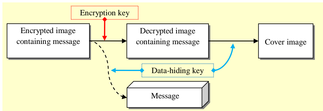
Fig. 3. Receiver in the RDHEI-2 framework
