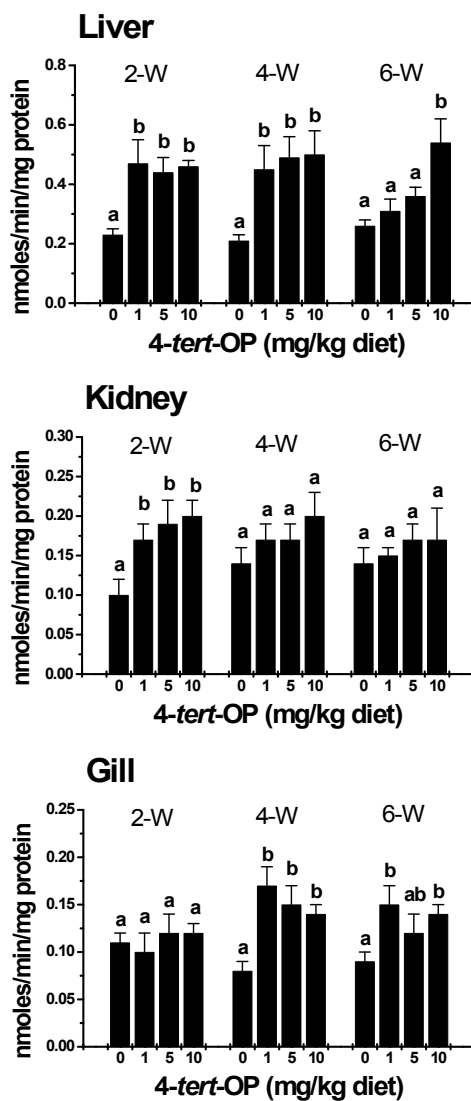
Fig. 4. Glutathione peroxidase enzyme activity (nmoles/min/mg protein) in liver, kidney and gill of olive flounder exposed to different levels of 4-tert-octylphenol for 2, 4 and 6 weeks. Data are represented as mean \pm S.E. ( n = 7 ). Columns with the same letter are not significantly different ( P > 0.05 ). Statistical comparison was made only within the groups of the same exposure period.
