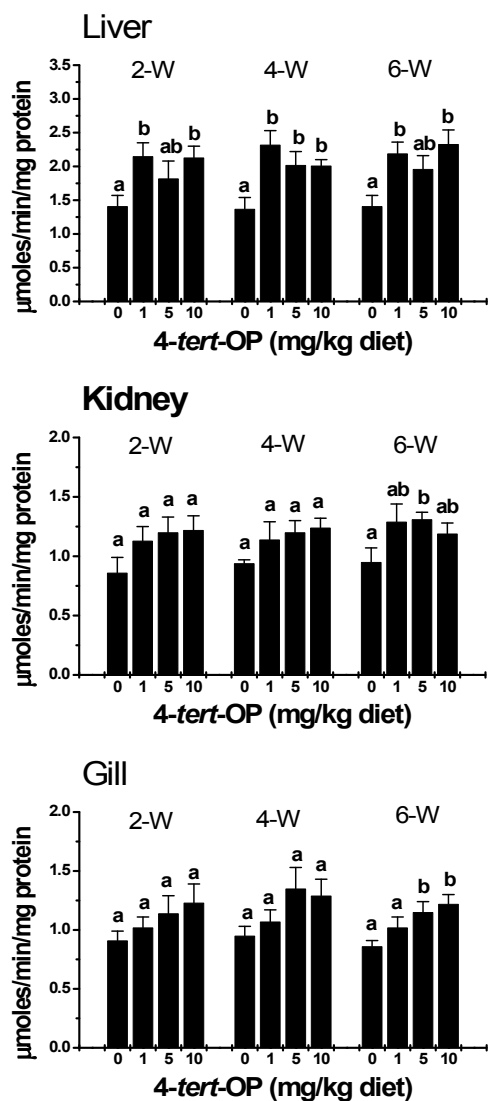
Fig. 3. Glutathione S-transferase enzyme activity ( \mu\text{moles}/\text{min}/\text{mg} protein) in liver, kidney and gill of olive flounder exposed to different levels of 4-tert-octylphenol for 2, 4 and 6 weeks. Data are represented as mean \pm S.E. ( n = 7 ). Columns with the same letter are not significantly different ( P > 0.05 ). Statistical comparison was made only within the groups of the same exposure period.
