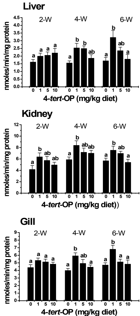
Fig. 2. Glutathione reductase enzyme activity (nmoles/min/mg protein) in liver, kidney and gill of olive flounder exposed to different levels of 4- tert -octylphenol for 2, 4 and 6 weeks. Data are represented as mean \pm S.E. ( n = 7 ). Columns with the same letter are not significantly different ( P > 0.05 ). Statistical comparison was made only within the groups of the same exposure period.
