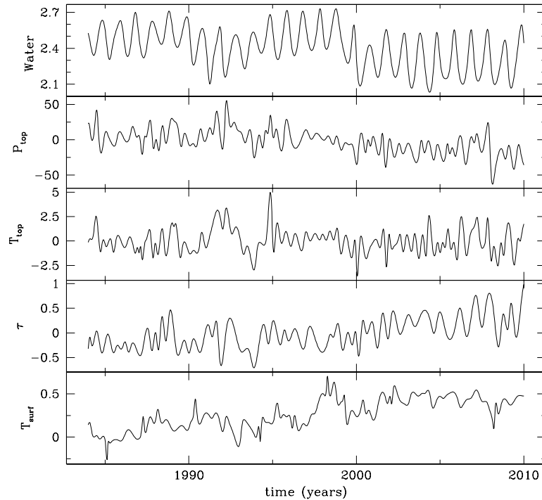
Fig. 3. Total column water vapor of cloud, cloud top pressure, cloud top temperature, cloud optical depth, and global surface air temperature from top to bottom panels, respectively.
