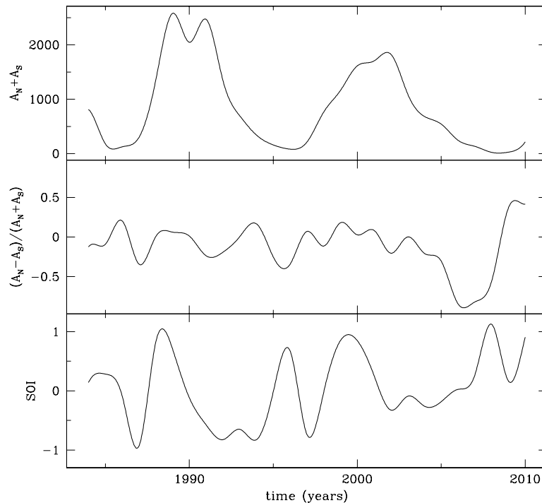
Fig. 1. Yearly total sunspot area, yearly solar north-south asymmetry, and yearly SOI index from top to bottom panels, respectively. SOI, Southern Oscillation Index.
