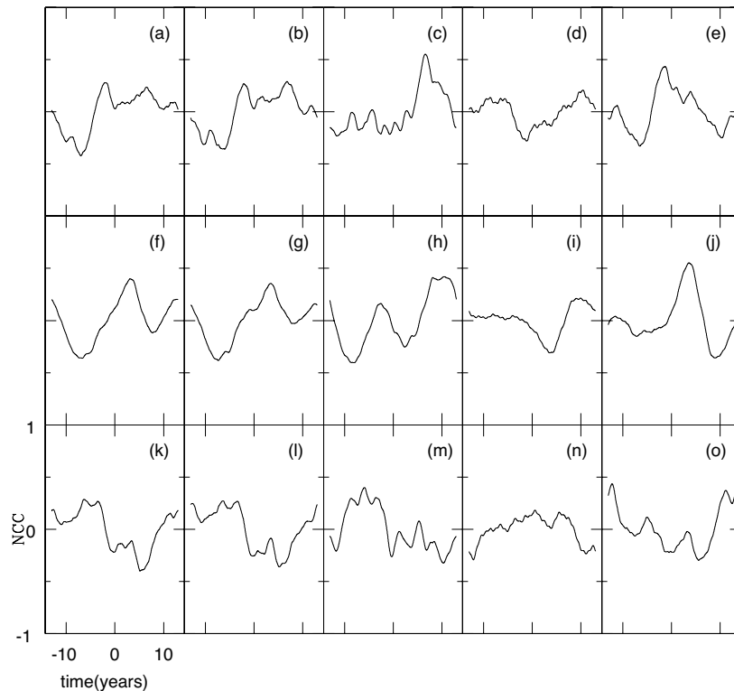
Fig. 4. Normalized cross-correlation resulting from the coverage of total cloud, cloud in the tropics, high-level cloud, medium-level cloud, and low-level cloud in columns from left to right, respectively. In the top, middle, and bottom rows, the normalized cross-correlations are calculated using the solar north-south asymmetry, total sunspot area, and the SOI index, respectively. SOI, Southern Oscillation Index.
