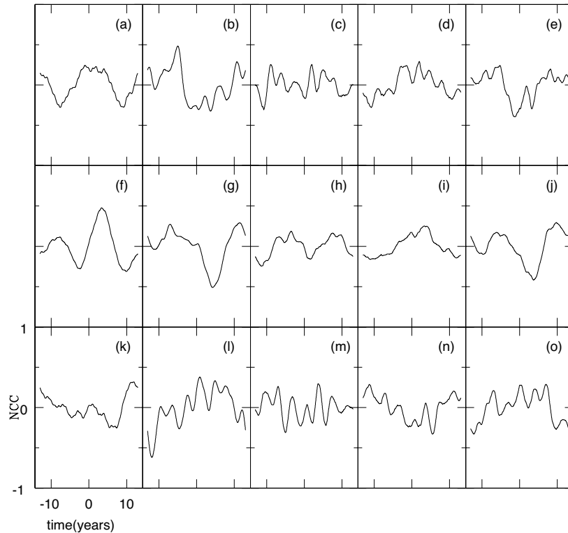
Fig. 5. Normalized cross-correlation resulting from the total column water vapor, global surface air temperature, top temperature, top pressure, and cloud optical depth in columns from left to right, respectively. In the top, middle, and bottom rows, the normalized cross-correlations are calculated using the solar north-south asymmetry, total sunspot area, and the SOI index, respectively. SOI, Southern Oscillation Index.
