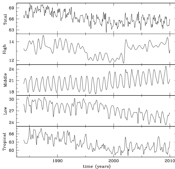
Fig. 2. Yearly coverage of clouds in terms of total cloud, high cloud, middle cloud, low cloud, and cloud in tropical regions (15°N–15°S) from top to bottom panels, respectively.
