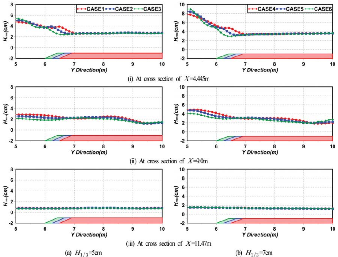
Fig. 8. Spatial distribution of simulated H_{rms} at three Y-Z cross sections.
