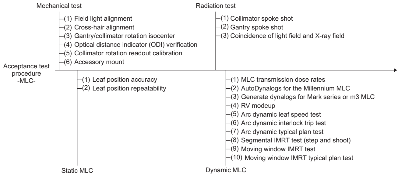
Fig. 4. The risk management items for acceptance test of external radiation therapy equipment: MLC.
