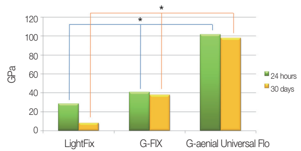
Fig. 3. Result of elastic modulus (Scheffe’s test). *: Significant differences were detected ( P < 0.05 ) in each materials.
