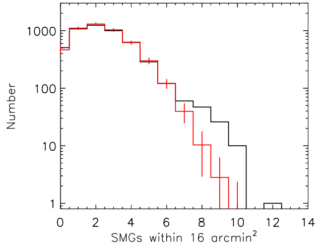
Figure 13. Histograms for number count of SMGs within a confined area. Black histogram represents the number of observed SMGs within an area of 4' \times 4' by positioning the area of 4' \times 4' randomly 5000 times. The same procedure was performed for uniformly distributed simulated SMGs (red histogram). The simulation was iterated 100 times using 100 simulated catalogs. Error bars represent the standard deviation of 100 iterations.
