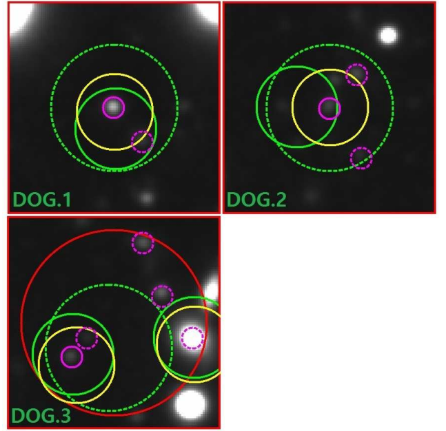
Figure 2. Post stamp images of three DOGs from Subaru/S-cam R_C band. The size of each stamp is 20'' \times 20'' . Symbols have the same meaning as in Figure 1. All optical objects (Oi et al. 2014) located within the beam size of PACS and SPIRE bands are identified with magenta symbols. The magenta solid line circle represents the DOG as well as the optical counterpart identified by LR analysis based on the mid-IR band. North is up, east is left.
