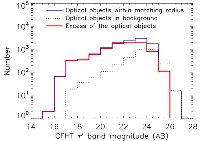
Figure 3. Various magnitude distributions of optical objects. The blue thin solid line is a distribution of objects within the matching radius around mid-IR objects, whereas the dotted line is a distribution of objects in the background. Subtraction of the two lines gives the red thick solid line, which results in q(m) after the normalization in Equation (3).
