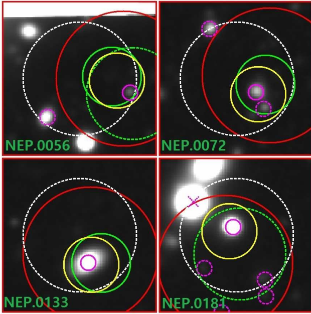
Figure 1. Post stamp images of four SMGs from Subaru/S-cam (Miyazaki et al. 2002) R_C band. The size of each stamp is 20'' \times 20'' . White, red, green (solid and dotted) and yellow circles represent FWHM of PSFs of SCUBA-2 850 \mu\text{m} , Herschel /SPIRE, Herschel /PACS ( 100 \mu\text{m} and 160 \mu\text{m} ) and AKARI mid-IR (L24) bands, which correspond to a diameter of 14''.8 , 17''.6 , 7''.7 , 12''.0 and 7''.2 , respectively. All optical objects (Oi et al. 2014) located within the beam size of 850 \mu\text{m} and SPIRE bands are identified with magenta symbols. The magenta solid line circle represents the optical counterpart identified by LR analysis based on mid-IR band data. The magenta 'x' represents an optical object that can be classified as a star candidate with the criteria of both stellarity ( >0.95 ) and u^*g'JKs color selection in Oi et al. (2014). The ID of each SMG comes from the 850 \mu\text{m} source catalog of Geach et al. (2017). North is up, east is left.
