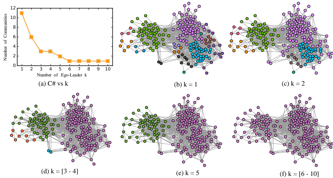
Fig. 5. Top-2 level Ego-Leader Sensitivity of parameter k on Jazz network.
