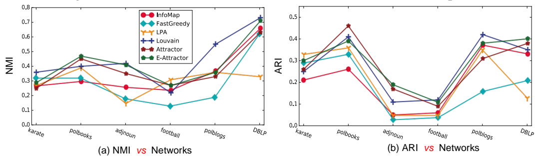
Fig. 7. Community detection performance of different algorithms on real-world networks.
