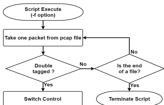
Fig. 9. Detection and Defense Module Flowchart
