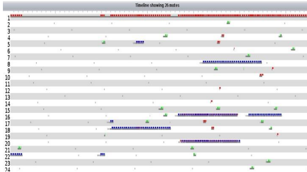
Fig. 5. Timeline showing the packets received per mote (node) over time.
