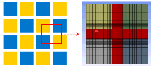
Figure 3. Modeling of DPF Channel.
