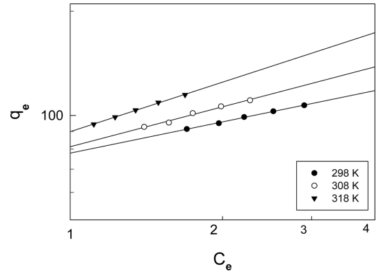
Fig. 3. Freundlich isotherms for brilliant green adsorption onto zeolite at different temperatures.
