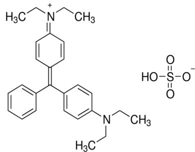
Fig. 1. Molecular structure of brilliant green.
