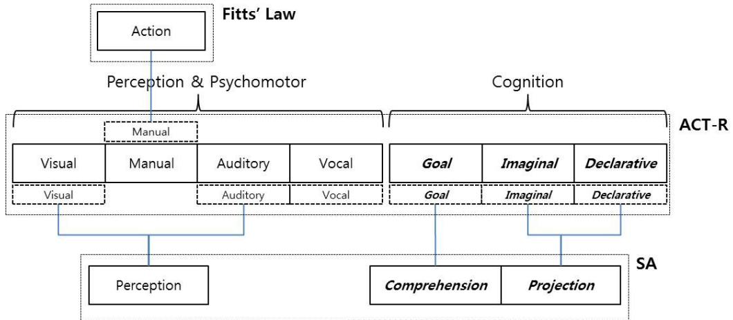
Fig. 7. The Representation of ACT-R Module Relations with SA & Fitts' Law
