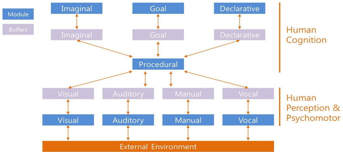
Fig. 2. Modular Representation of ACT-R Cognitive Architecture
