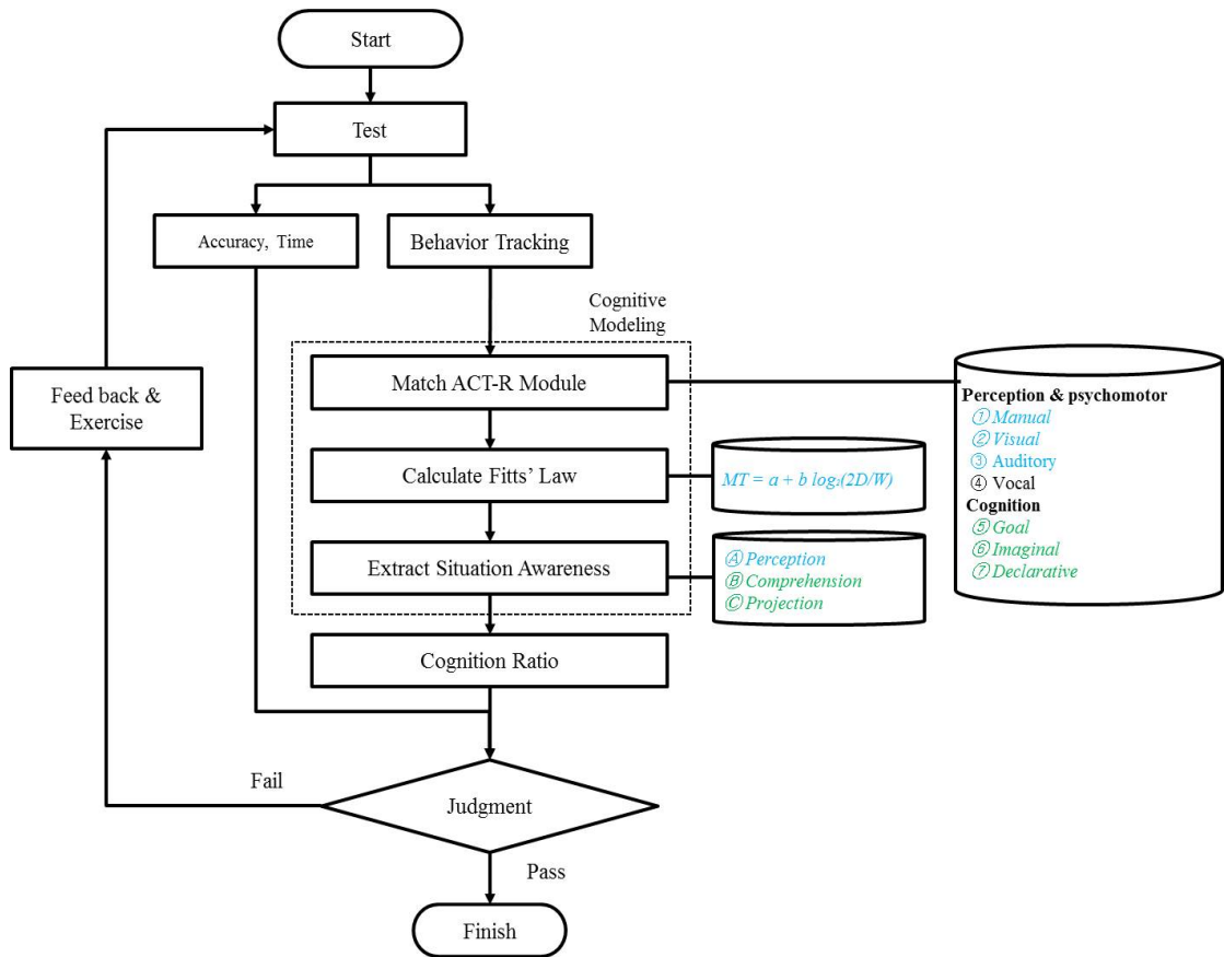
Fig. 8. The Concept of Situation Awareness Assessment Model Using Cognitive Architecture
