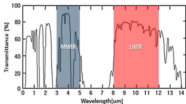
Fig. 1. atmospheric window
