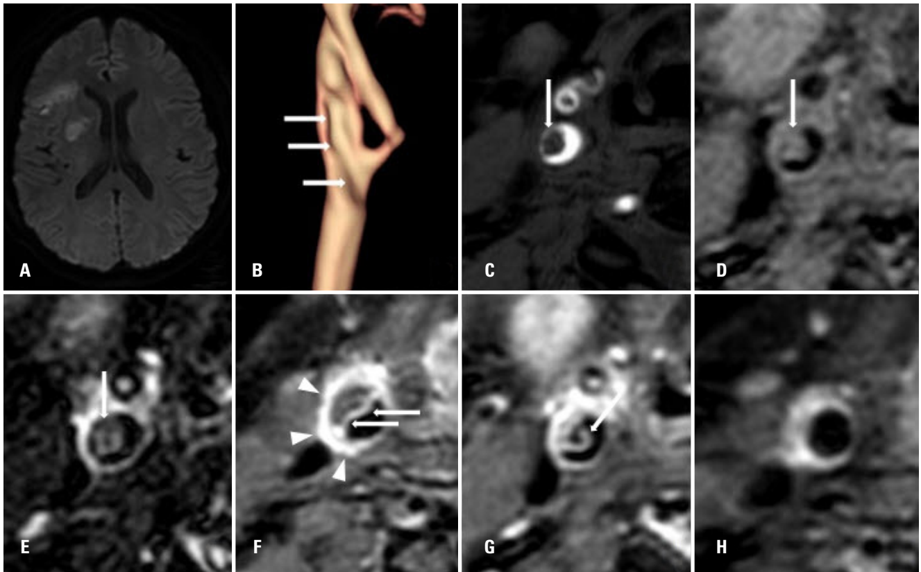
Fig. 1. A 50-year-old woman with a transient left-side weakness and mild dysarthria. (A) Diffusion-weighted imaging showing multifocal infarctions in the right basal ganglia, frontal cortex, and parietal cortex. (B) Volume-rendering imaging showing a filling defect in the long segment of the CCA and ICA (arrows). (C) Axial source image of time-of-flight carotid MRA showing a massive intraluminal filling defect in the right CCA (arrow). (D) Axial image of nonenhanced T1-weighted carotid MRI showing the intravascular thrombus without an intramural plaque or intimal flap (arrow). (E) Axial image of nonenhanced T2-weighted carotid MRI showing the intravascular thrombus without an intramural plaque or intimal flap (arrow). (F) Contrast-enhanced MRI of the right CCA showing the circumferential enhancement (arrowheads) with a mural wall thrombus (arrows). (G) Contrast-enhanced MRI of the right ICA showing the intimal disruption (arrow). (H) Contrast-enhanced axial imaging performed 10 days after the initial carotid plaque MRI showing complete resolution of the mural wall thrombus and intimal disruption and a marked decrease in the circumferential carotid wall enhancement. CCA, common carotid artery; ICA, internal carotid artery; MRA, magnetic resonance angiography; MRI, magnetic resonance imaging.
