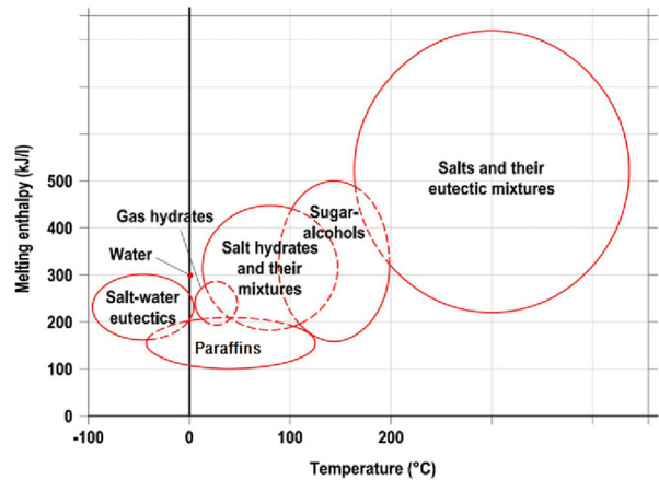
Figure 2. Melting enthalpy vs. phase-change temperature for various materials used in PCMs (Baetens et al., 2010).
