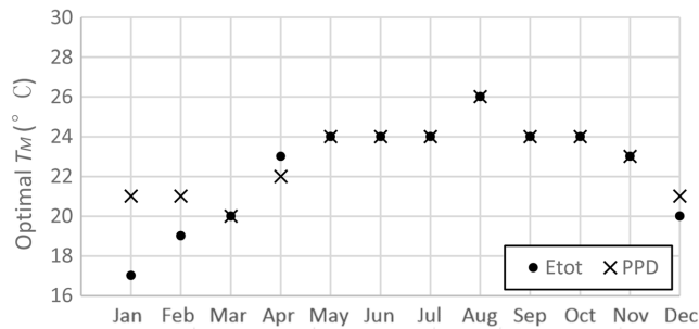
Figure 10. Monthly optimal T_M in terms of E_{tot} and PPD.
