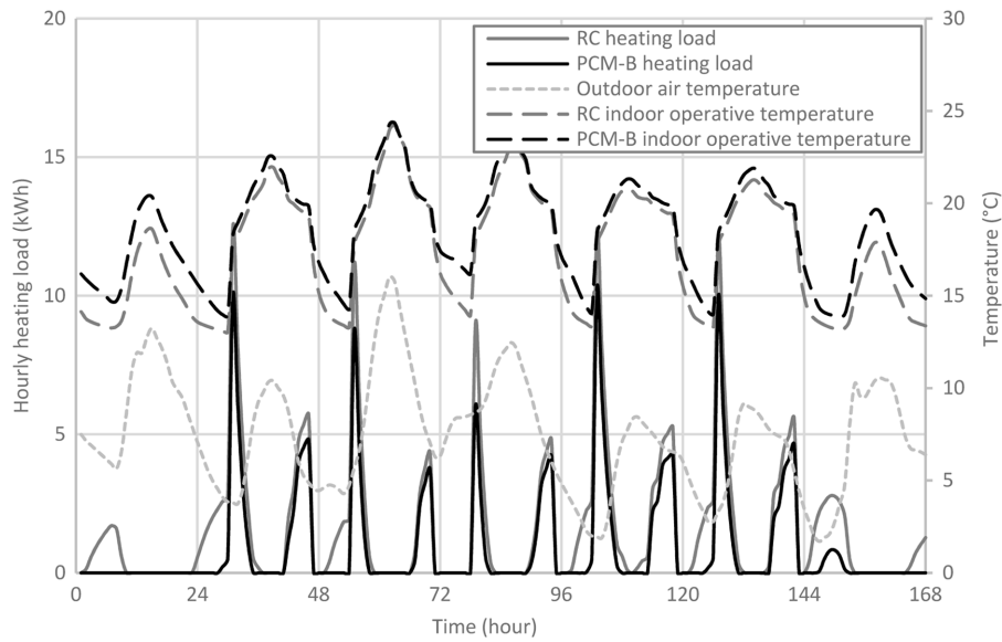
Figure 11. Hourly heating load and indoor operative temperature of RC and PCM-B ( T_M = 22^\circ\text{C} ) for a south-oriented cellular office room with \text{WWR} = 40\% in Dec 3-9.
