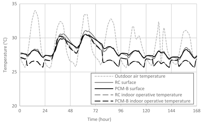
Figure 9. Comparison of the façade inner surface temperature and indoor operative temperature of RC and PCM-B ( T_M=22^{\circ}\text{C} ) for a south-oriented cellular office room with WWR = 40% in Aug 4-10.
