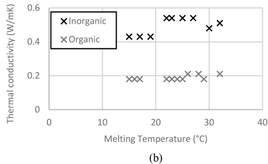
Figure 3. (a) Latent heat capacity vs. melting temperature (b) thermal conductivity vs. melting temperature of commercially available PCM products from a manufacturer (Phase Change Material Products Ltd., 2016).
