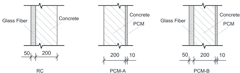
Figure 5. Constructions of the three configurations (Unit: mm).
