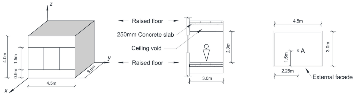
Figure 4. Cellular office room model.
