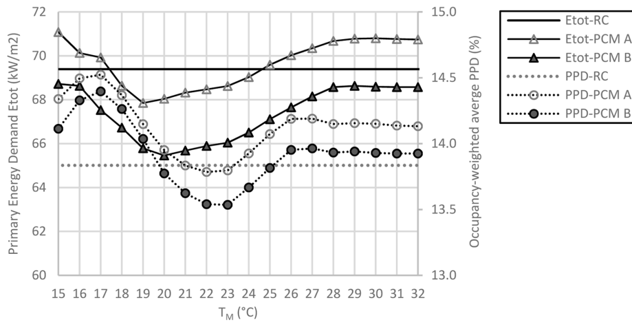
Figure 6. Primary energy demand and occupancy-weighted average PPD vs. T_M for RC, PCM-A, and PCM-B for a south-oriented cellular office room with WWR = 40%.
