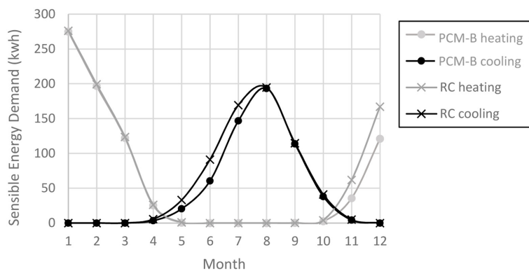
Figure 7. Monthly heating and cooling sensible energy demands of RC and PCM-B ( T_M = 22^\circ\text{C} ) for a south-oriented cellular office room with WWR = 40%.
