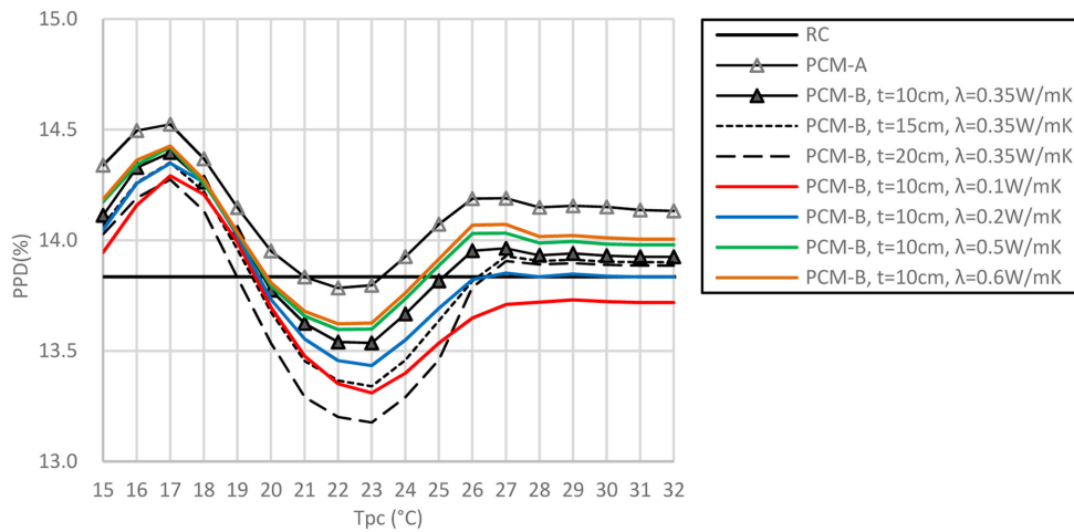
Figure 13. Sensitivity of thickness and thermal conductivity of PCM layer to thermal discomfort.
