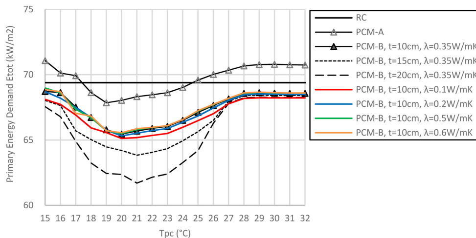
Figure 12. Sensitivity of thickness and thermal conductivity of PCM layer to total energy demand.
