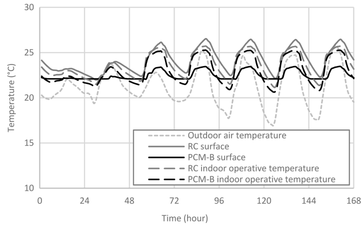
Figure 8. Comparison of the façade inner surface temperature and indoor operative temperature of RC and PCM-B ( T_M=22^{\circ}\text{C} ) for a south-oriented cellular office room with WWR = 40% from June 3-9.
