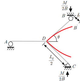
Fig. 5. Deformation of members due to overturning moment
