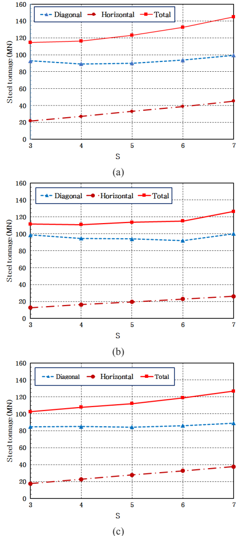
Fig. 11. Steel tonnage for hexagrid members (S=4) (a)HS-1 (b)HS-2 (c)HS-3
