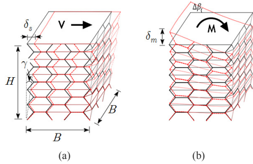
Fig. 7. Deformation of hexagrid unit (a) Shear (b) Flexural
