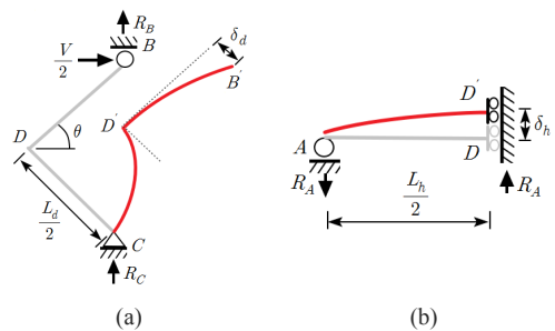
Fig. 3. Deformation of members due to shear (a)diagonal (b)horizontal
