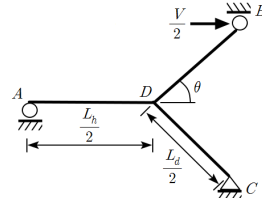
Fig. 2. Behavior of repetitive unit cell for shear
