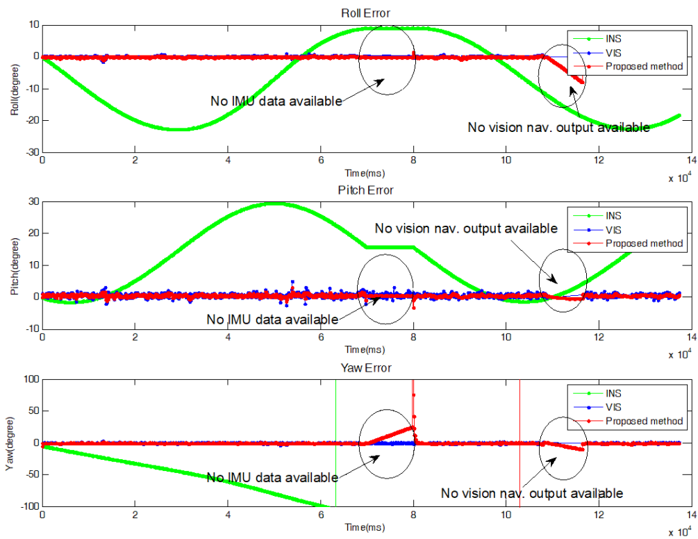
Fig. 10. Attitude error in simulation.
