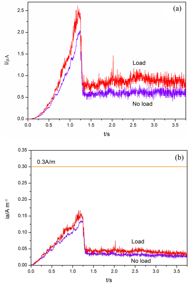
Fig. 2 Current transients (a) and pit stability products (b) of metastable double pits of stainless steel under loading and no loading at R_t=1.25s and D_0=5.0\times 10^{-5} cm^2/s .
