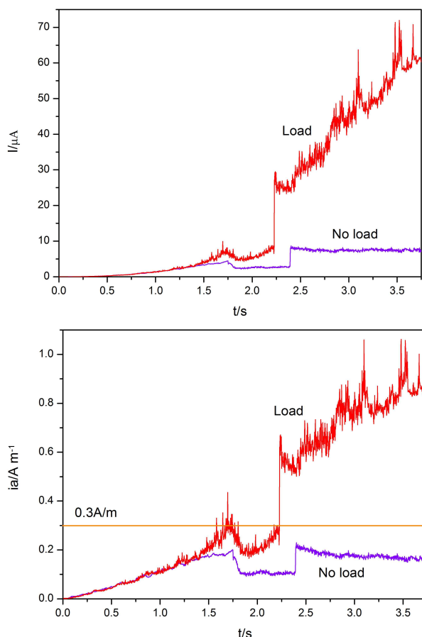
Fig. 3 Current transients (a) and pit stability products (b) for metastable double pits at R_f=1.75\text{s} and D_0=5.0 \times 10^{-5} \text{ cm}^2/\text{s} .
