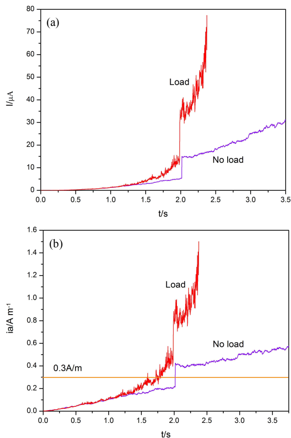
Fig. 4 Current transients (a) and pit stability products (b) for metastable double pits at R_f=1.25\text{s} and D_0=8.0 \times 10^{-7} \text{ cm}^2/\text{s} .
