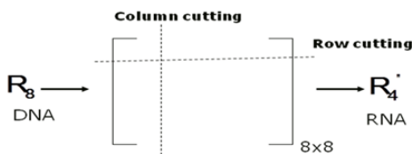
(b) R_8 DNA to R_4'' RNA [6] .
