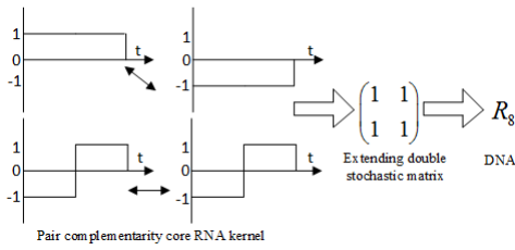
(a) R_4'' RNA to R_8 DNA.
