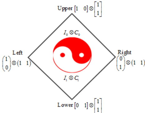
(b) R_8 DNA to R_4'' RNA [6] .
