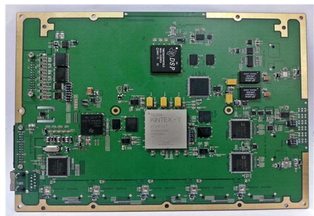
Fig. 4. PCB of a digital module.
