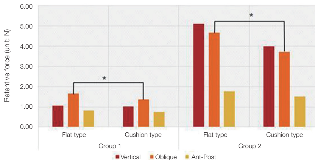
Fig. 4. Comparison of retentive force according to the type of magnetic attachment.
