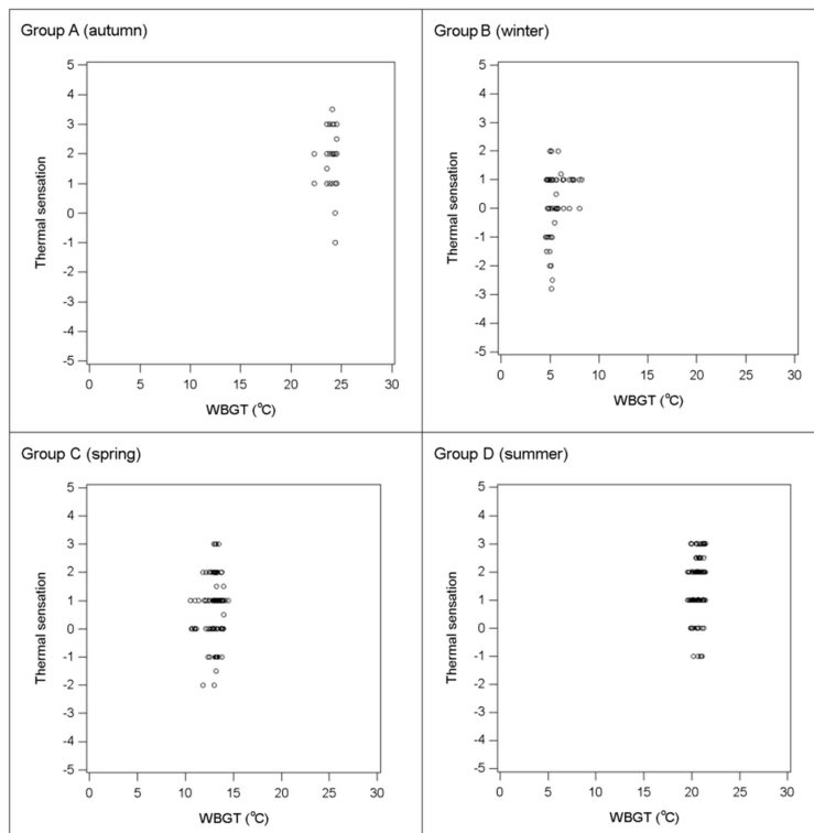
Figure 4. Thermal sensation and WBGT for 60 minutes (see chapter 2.5)
