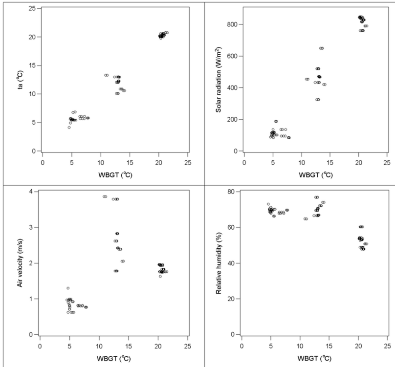
Figure 3. Weather data at 3m and WBGT for Groups B, C, and D
