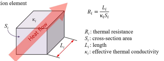
Fig. 3. Thermal resistance R_i
