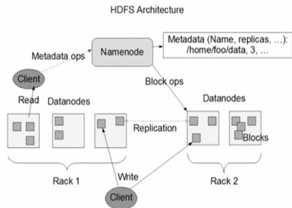
Fig. 1. HDFS Architecture
