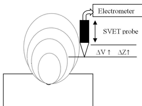
Fig. 4 Schematic diagram of the movement of scanning vibrat electrode probe across the equi-potential lines.
