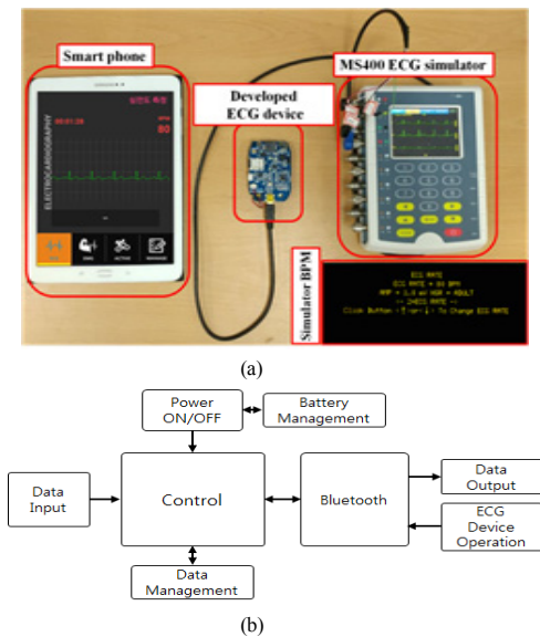
Fig. 9. Developed mobile ECG measurement system (a) Android smart device, Developed ECG Measurement system, MS400(ECG Simulator) (b) Block diagram for Developed ECG Measurement system
