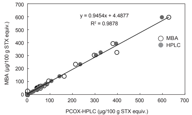
Fig. 3. Correlation between mouse bioassay and post-column oxidation-high performance liquid chromatography (HPLC) method.
