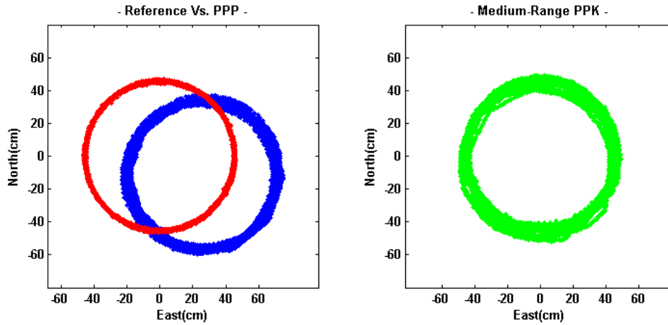
Fig. 8. Horizontal trajectories of the turn-table test: the left graph depicts comparison of the PPP (blue colored) with the reference (red colored), whereas the right graph presents that of the medium-range PPK.
