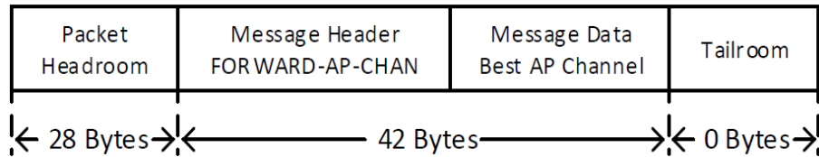
Fig. 4. Format of protocol message FORWARD-AP-CHAN
