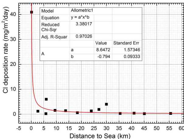
Fig. 5. Variation of chloride deposition rate as a function of the distance to sea (based on data 13) in Table 2).
